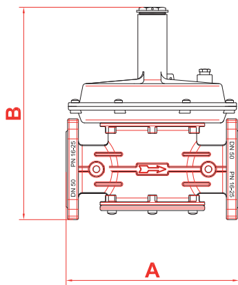
Versions with flanged connections
