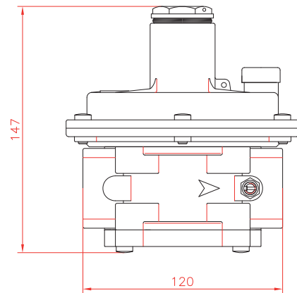
Overall dimensions in mm STANDARD version IRN3/IRN5
