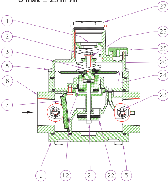
IRC3 / IRC5 COMPACT version Q max = 25 m 3 /h
