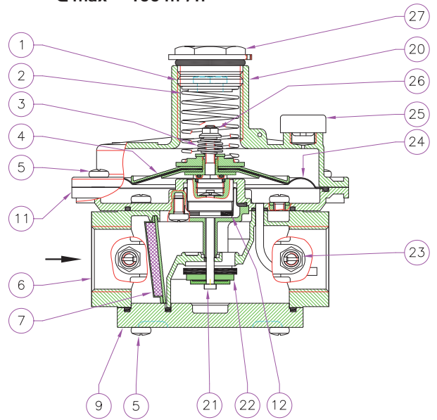
IRN3 / IRN5 STANDARD version Q max = 100 m 3 /h
