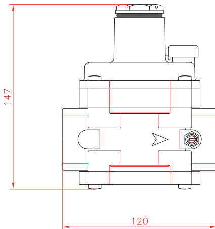
Overall dimensions in mm COMPACT version IRC3/IRC5
